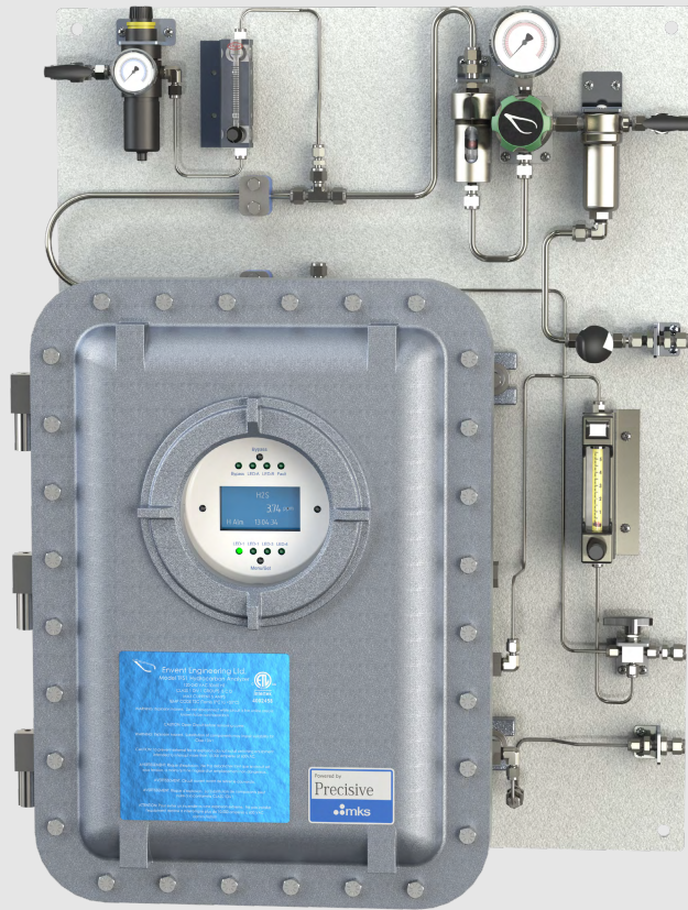
TFS1-EX HYDROCARBON ANALYZER SHOWN WITH A SAMPLE CONDITIONING SYSTEM FOR SATURATED & DIRTY GAS
